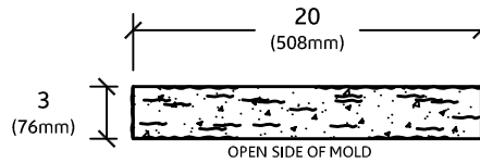
ELEVATION VIEW
