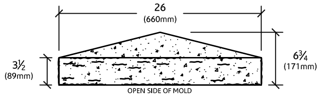
ELEVATION VIEW
