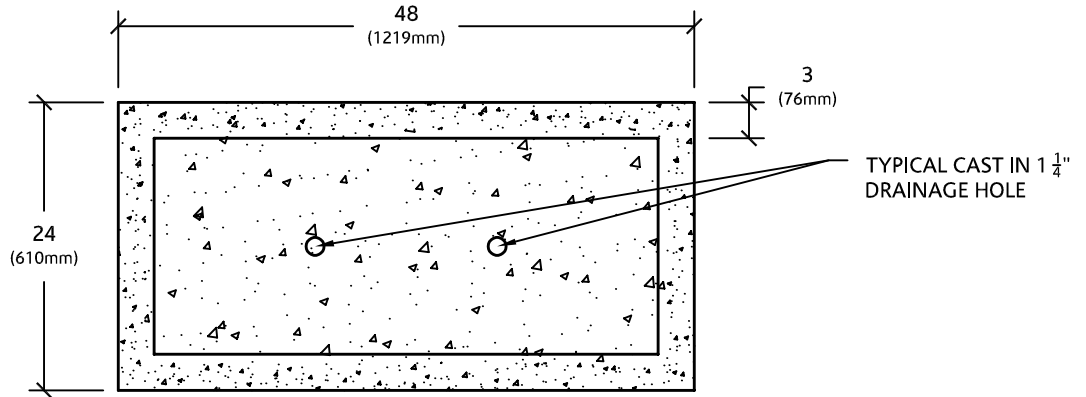
PLAN VIEW
