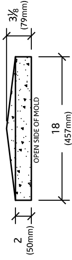
ELEVATION VIEW
