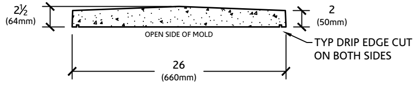
SECTION VIEW
