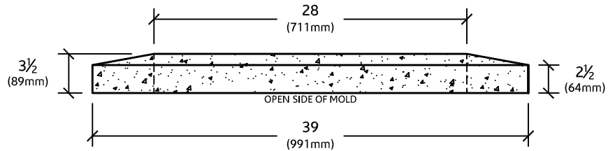
ELEVATION VIEW
