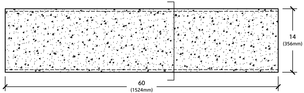
PLAN VIEW
