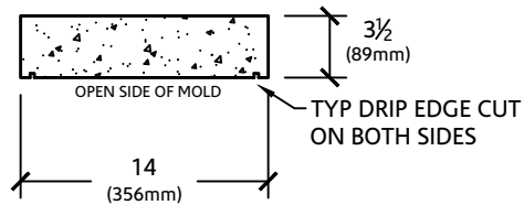
SECTION VIEW
