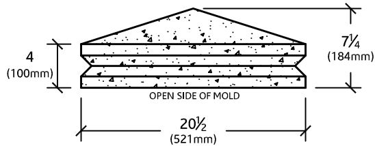
ELEVATION VIEW
