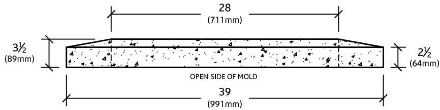
ELEVATION VIEW
