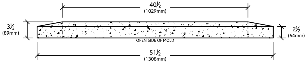
ELEVATION VIEW
