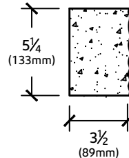
SECTION VIEW
