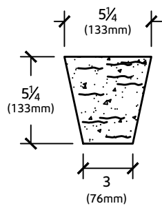
ELEVATION VIEW
