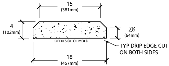
SECTION VIEW
