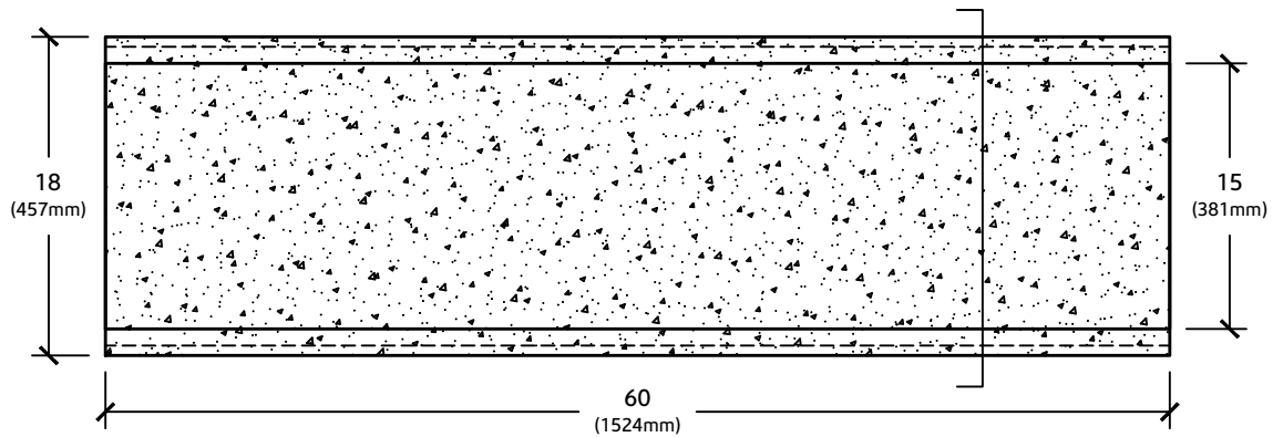
PLAN VIEW
