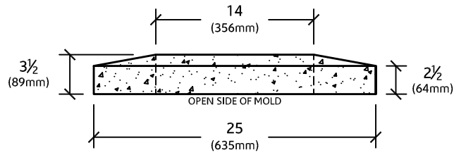
ELEVATION VIEW
