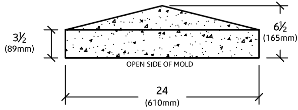
SECTION VIEW
