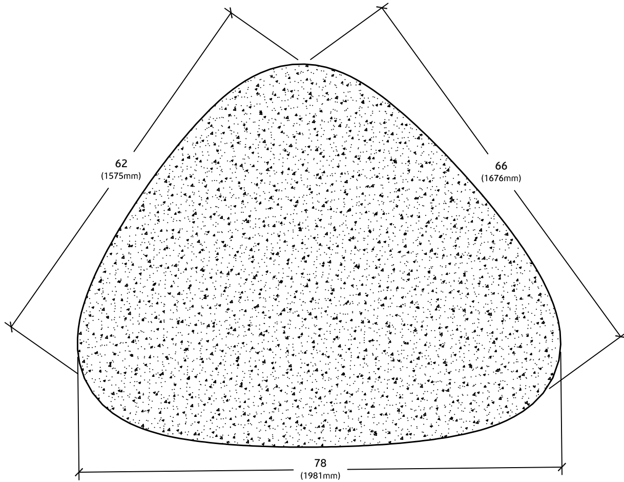
PLAN VIEW
