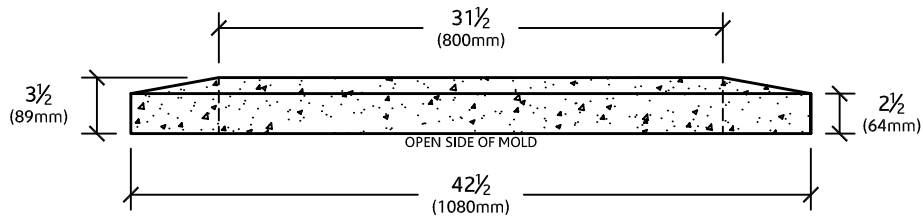
ELEVATION VIEW
