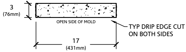
SECTION VIEW
