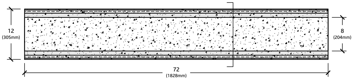
PLAN VIEW
