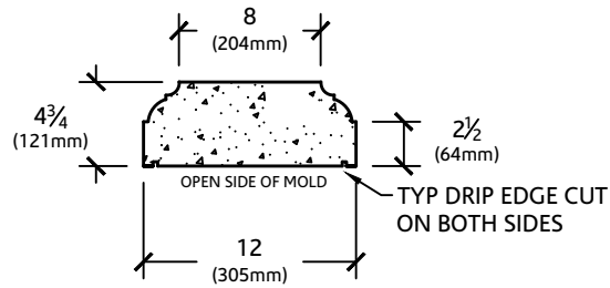
SECTION VIEW
