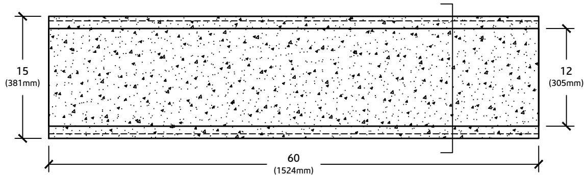
PLAN VIEW
