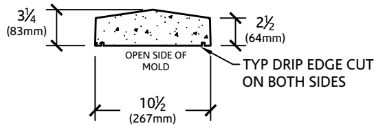
SECTION VIEW
