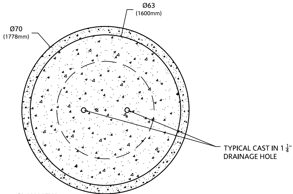
PLAN VIEW
