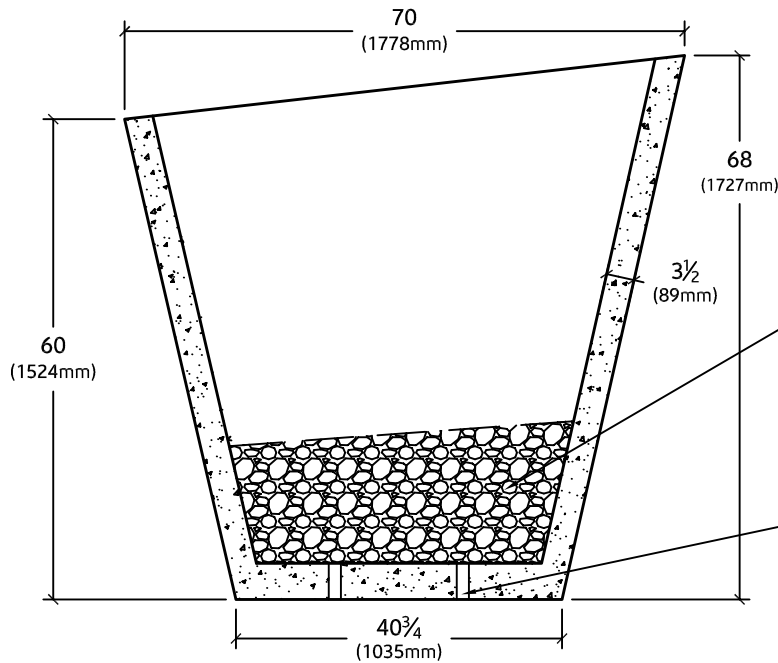
SECTION VIEW
