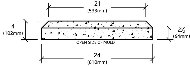
ELEVATION VIEW
