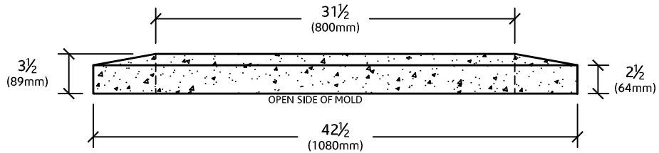
ELEVATION VIEW
