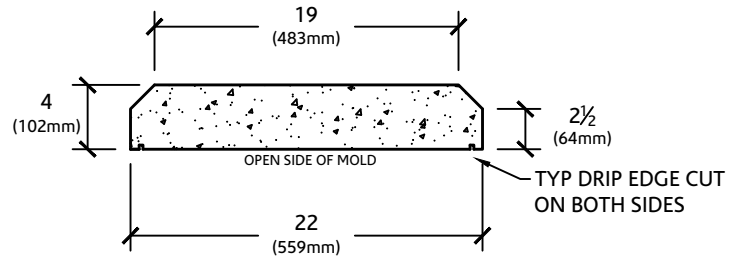
SECTION VIEW
