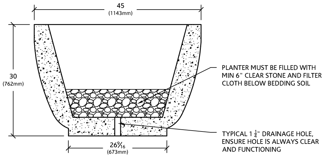
SECTION VIEW
