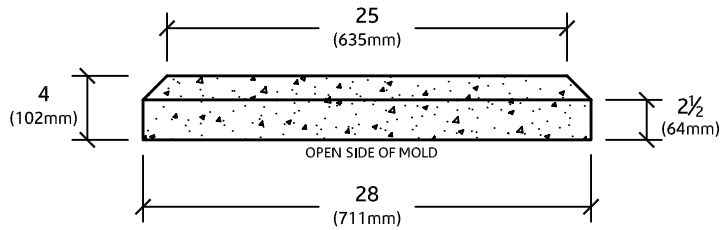
ELEVATION VIEW
