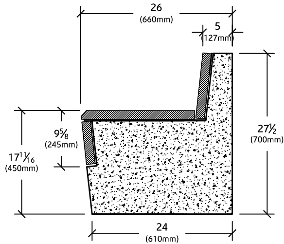
SECTION VIEW
