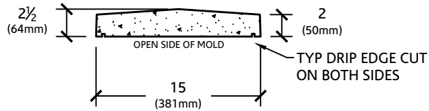
SECTION VIEW
