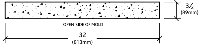
ELEVATION VIEW
