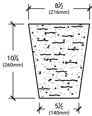
ELEVATION VIEW
