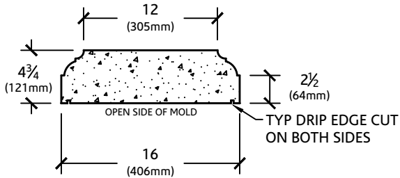
SECTION VIEW
