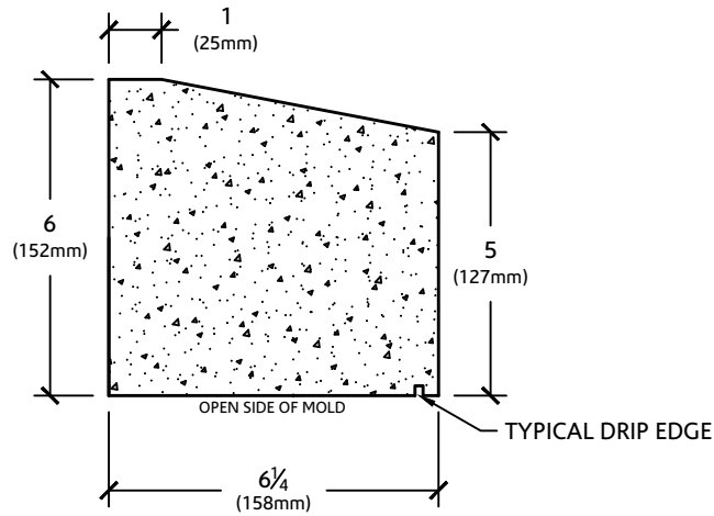
SECTION VIEW
