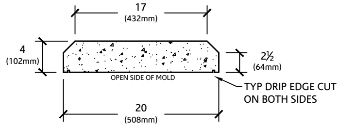
SECTION VIEW
