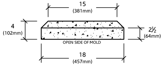
ELEVATION VIEW
