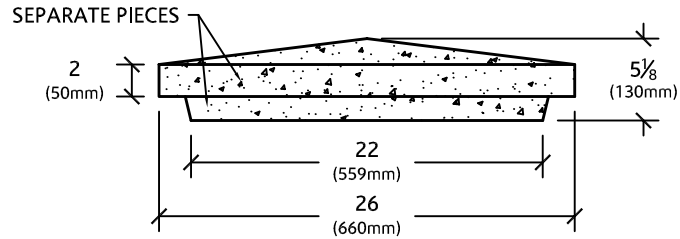
ELEVATION VIEW
