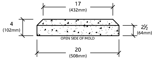
ELEVATION VIEW
