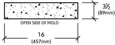
ELEVATION VIEW
