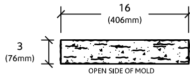
ELEVATION VIEW
