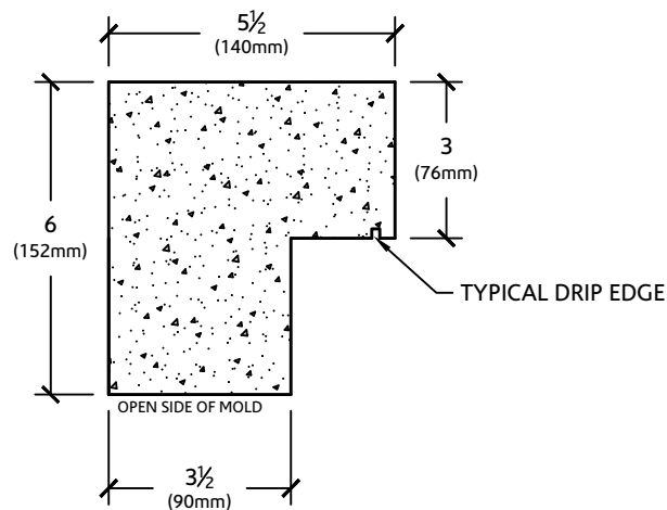
SECTION VIEW
