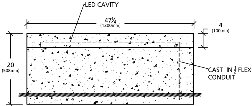
ELEVATION VIEW
