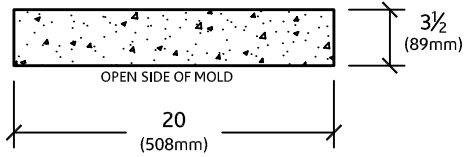
ELEVATION VIEW
