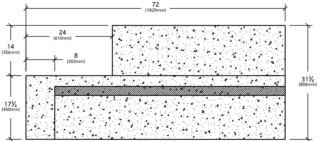
ELEVATION VIEW
