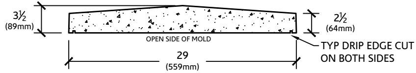
SECTION VIEW
