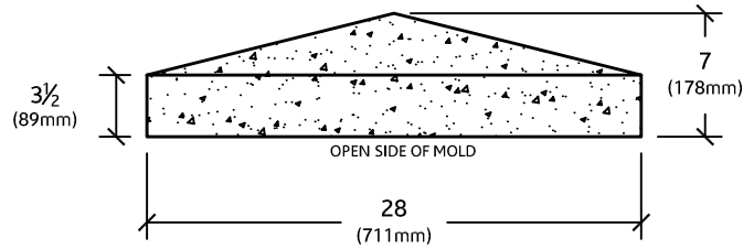
ELEVATION VIEW
