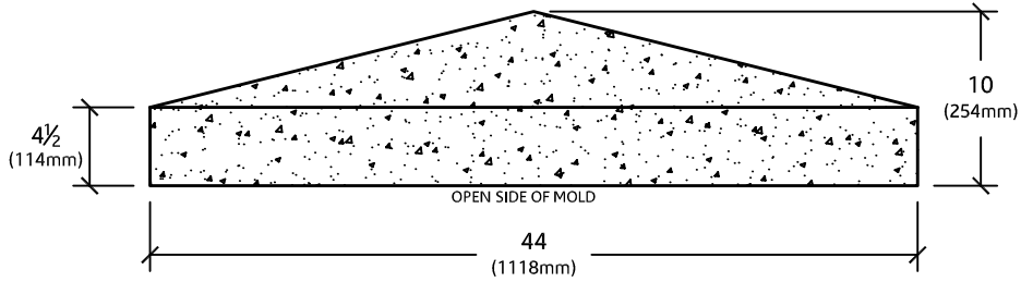
SECTION VIEW
