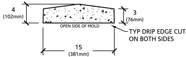
SECTION VIEW
