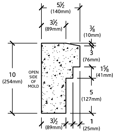
SECTION VIEW
