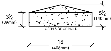
ELEVATION VIEW
