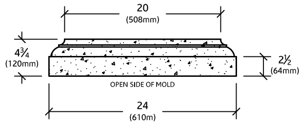
ELEVATION VIEW
