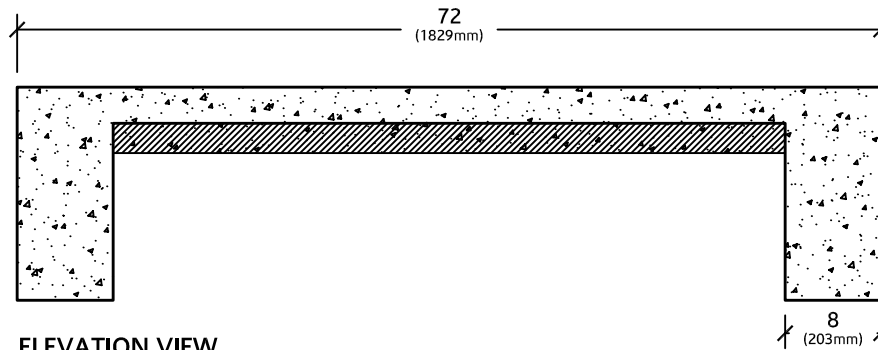
ELEVATION VIEW
